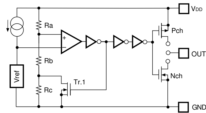
FIG. 1 Block Diagram
