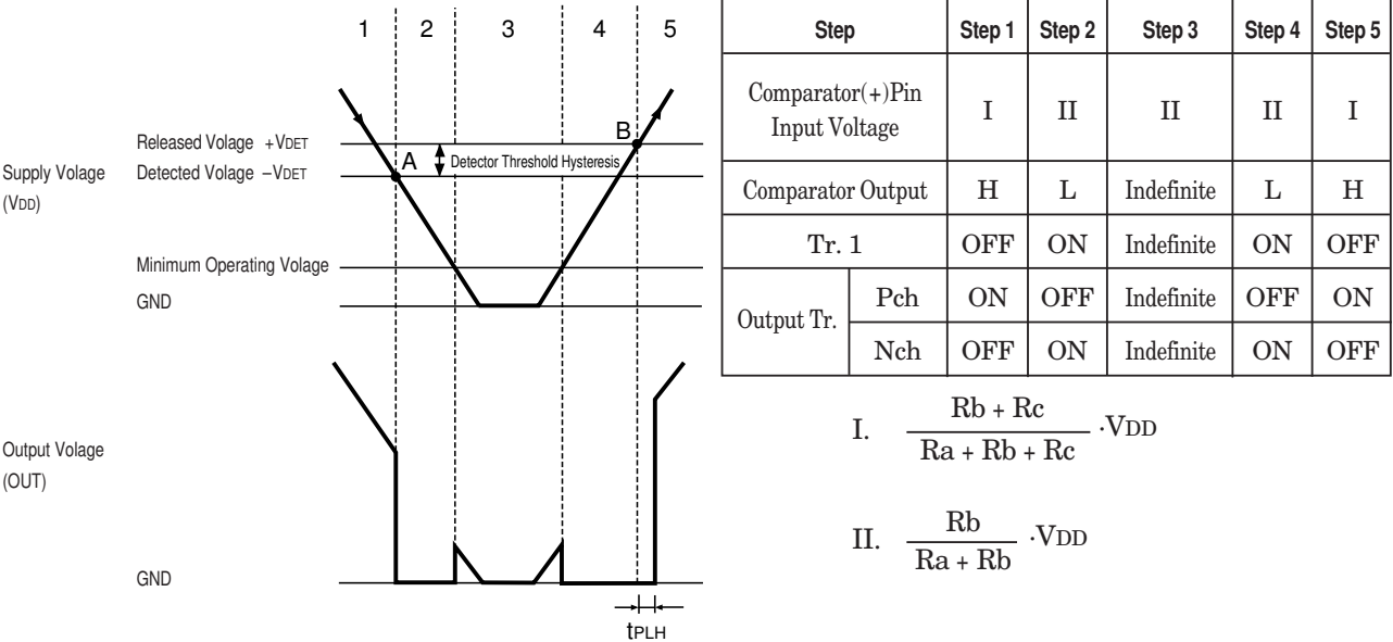
FIG. 2 Operation Diagram
