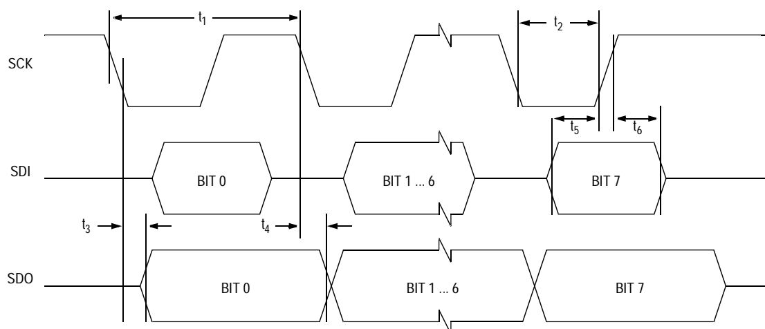
Figure 14-1. SIOPI Timing Diagram
