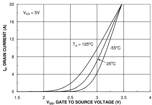
Figure 5. Transfer Characteristics.
