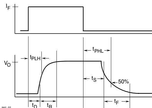
Figure 2. Non-saturated Switching Timing
