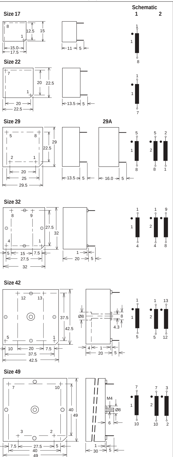
Mounting Style F
