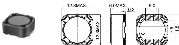
Dimensions (mm)
