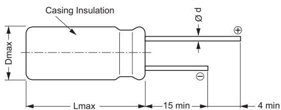
5 \leq \text{ØD} \leq 18 Long leads EKO 00...
