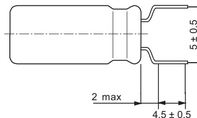
5 \leq \text{ØD} \leq 8 Leads bent open, shortened EKO 09... (S = 5mm)
