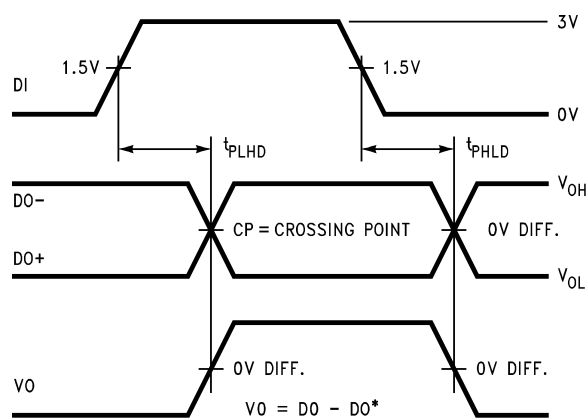
FIGURE 3. Driver Differential Propagation Delay Timing
