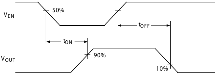
Active-Low Switch Delay Times (MIC20x6-2)
