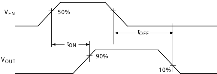
Active-High Switch Delay Times (MIC20x6-1)
