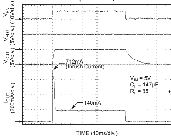
Turn-On/Turn-Off (MIC2026-1)
