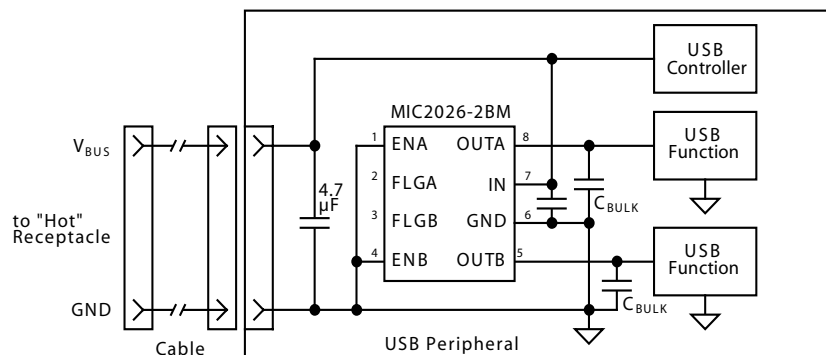
Figure 3. Hot-Plug Application
