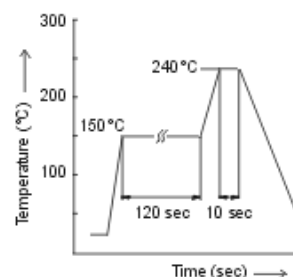
soldering condition
