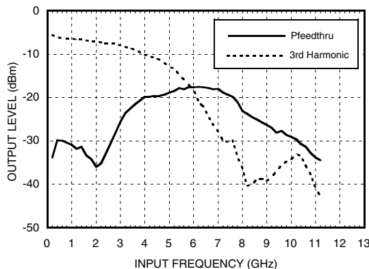
Output Harmonic
