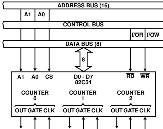
FIGURE 4. 82C54 SYSTEM INTERFACE
