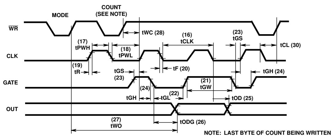
FIGURE 20. CLOCK AND GATE
