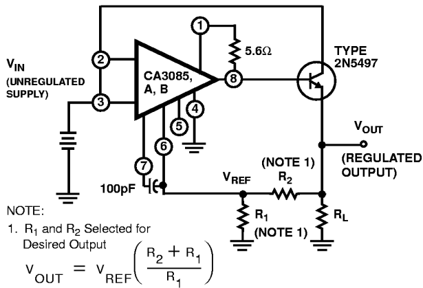
FIGURE 17. TYPICAL HIGH CURRENT VOLTAGE REGULATOR CIRCUIT
