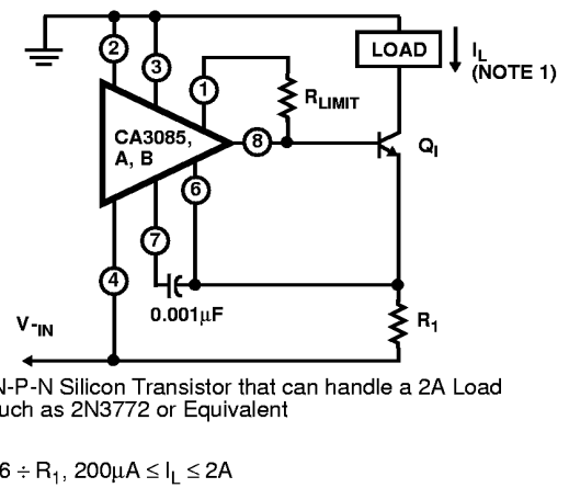
FIGURE 18. TYPICAL CURRENT REGULATOR CIRCUIT
