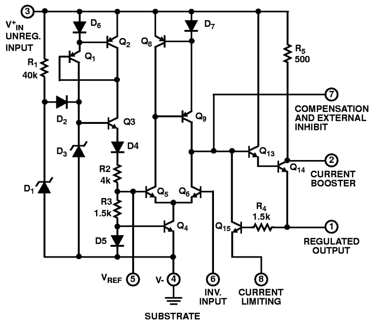
FIGURE 1. SCHEMATIC DIAGRAM OF CA3085 SERIES
