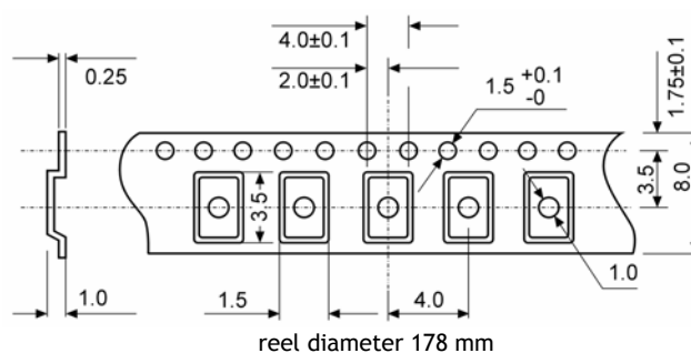
tape specification
