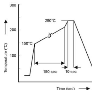
soldering condition
