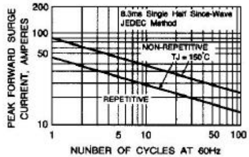
Fig. 2-MAXIMUM PEAK FORWARD SURGE CURRENT
